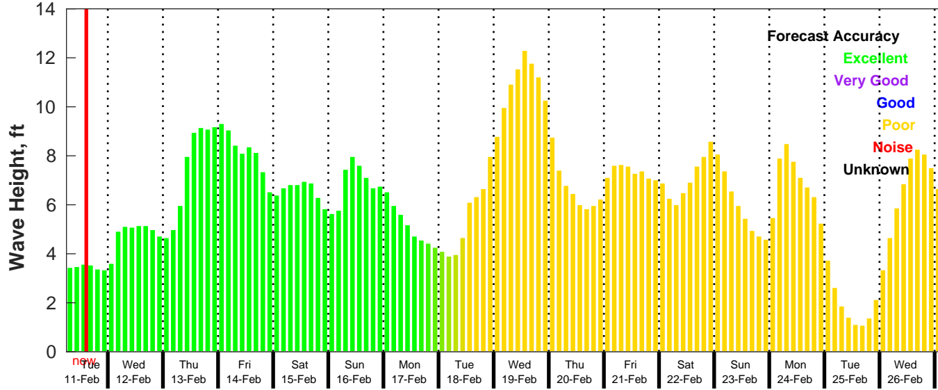
GFS Wave Forecast for NDBC 42019 from 11-Feb-2025 06:00:00 to 27-Feb-2025 06:00:00
