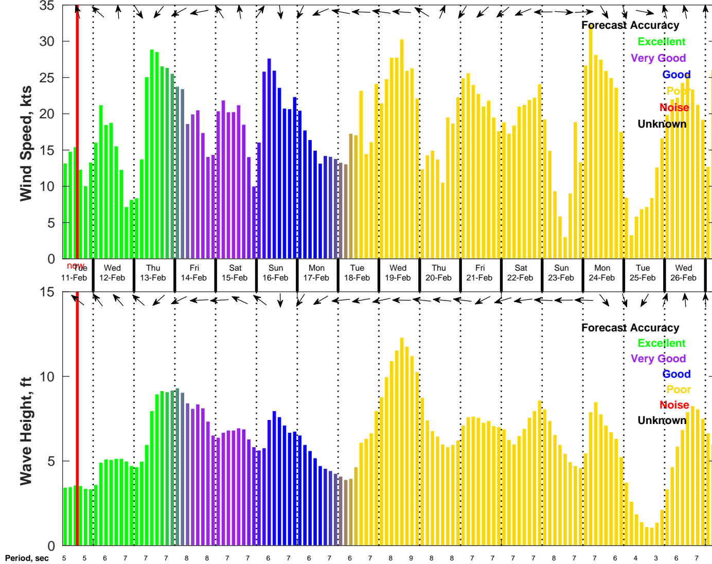
Wind & Wave Forecast for NDBC 42019 from 11-Feb-2025 06:00:00 to 27-Feb-2025 06:00:00
