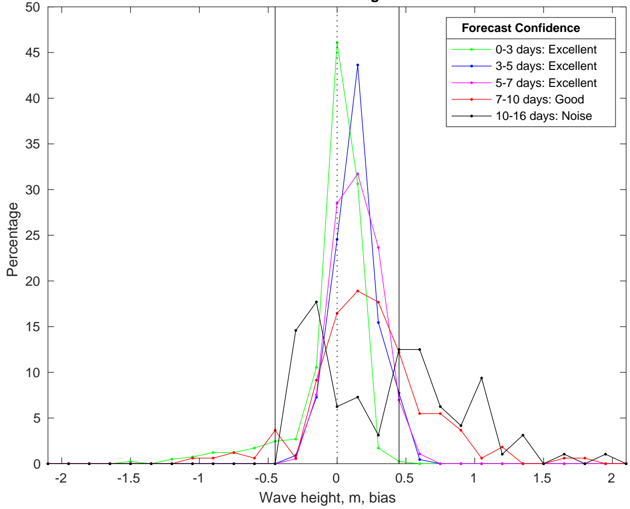
NDBC 42020 vs GFS Waves Bias Histogram: 11-Feb-2025
