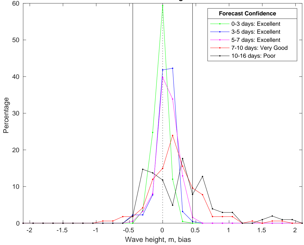
NDBC 42035 vs GFS Waves Bias Histogram: 11-Feb-2025
