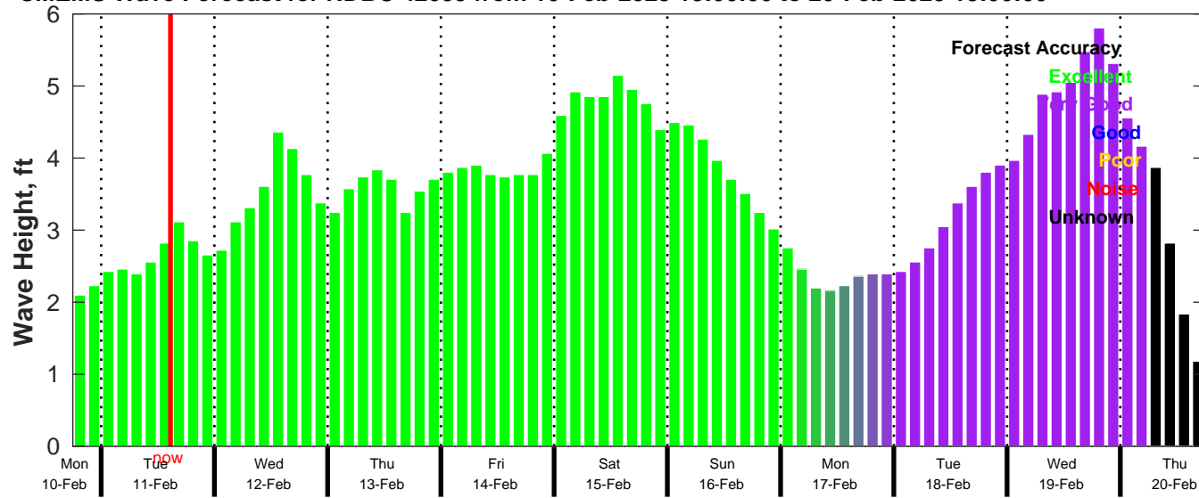
CMEMS Wave Forecast for NDBC 42035 from 10-Feb-2025 18:00:00 to 20-Feb-2025 18:00:00
