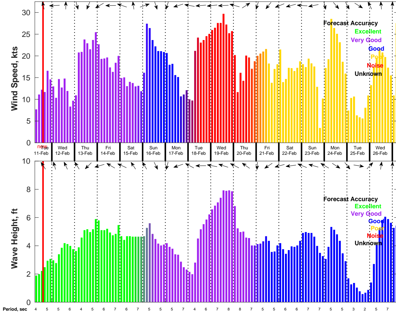
Wind & Wave Forecast for NDBC 42035 from 11-Feb-2025 06:00:00 to 27-Feb-2025 06:00:00
