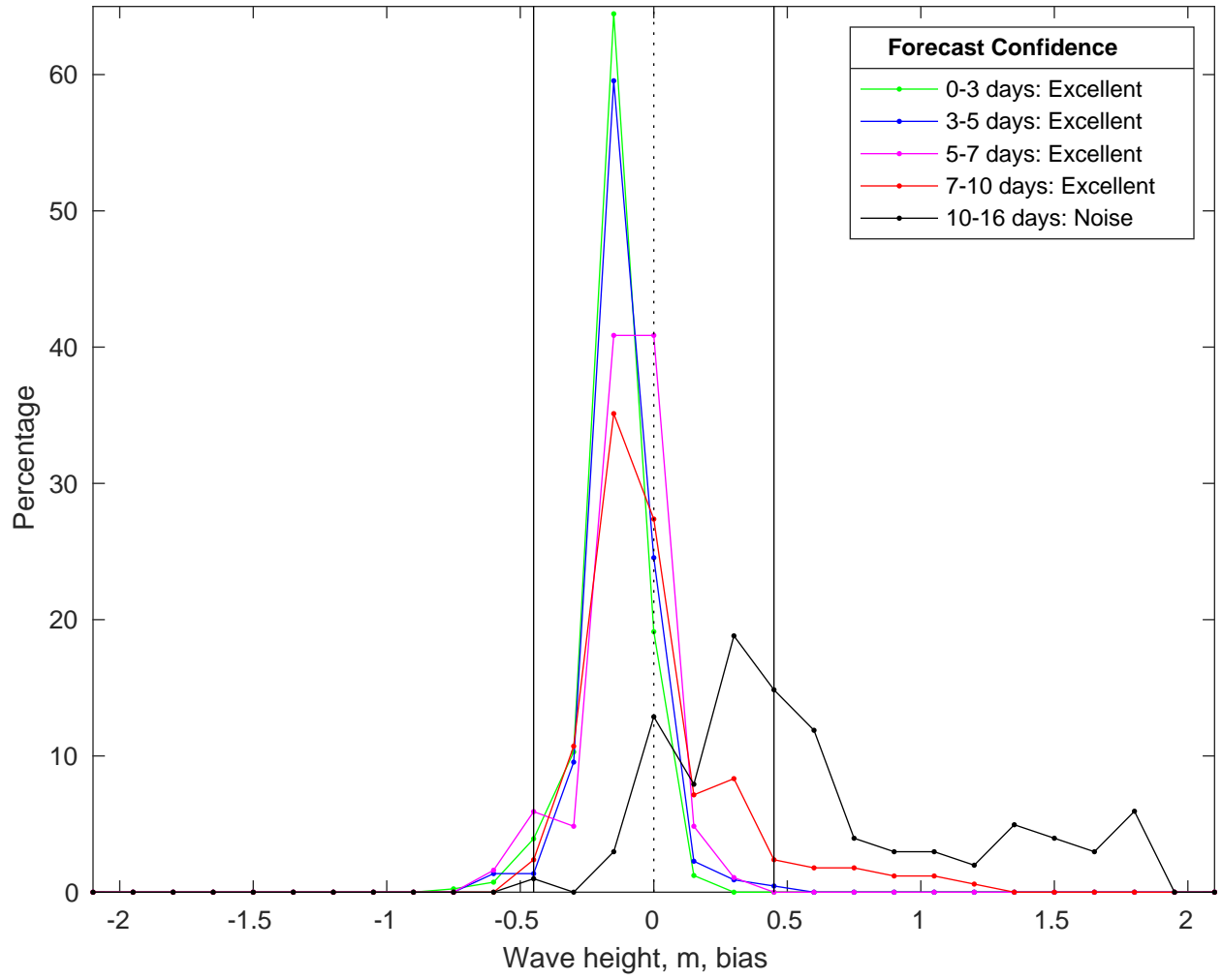
NDBC 42036 vs GFS Waves Bias Histogram: 11-Feb-2025
