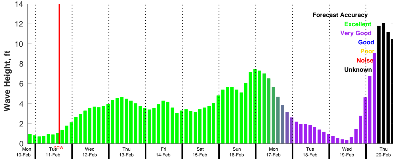
CMEMS Wave Forecast for NDBC 42036 from 10-Feb-2025 19:00:00 to 20-Feb-2025 19:00:00
