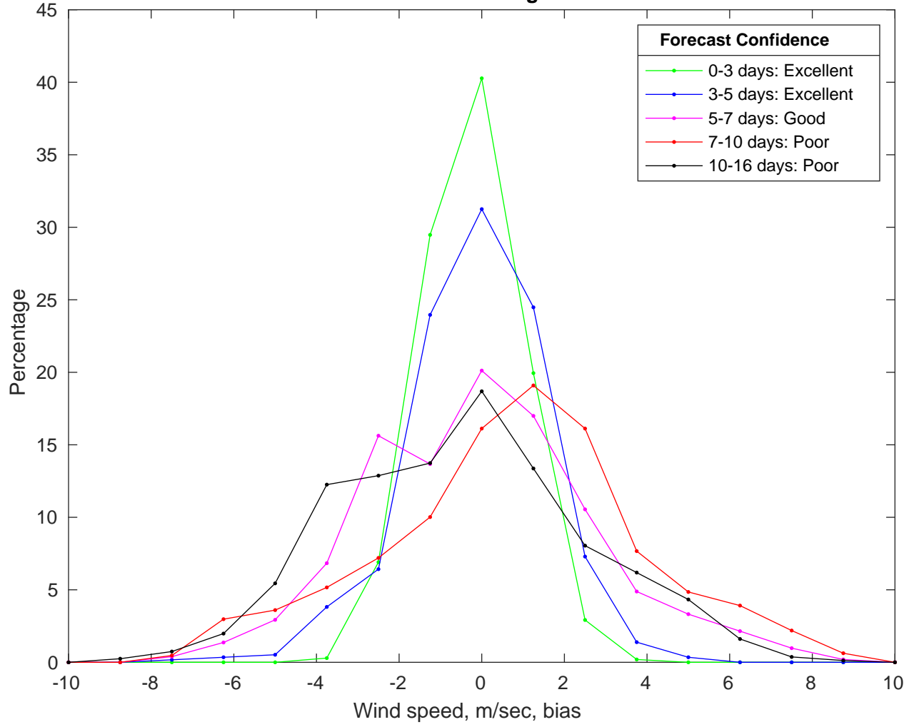
NDBC 42036 vs GFS Winds Bias Histogram: 26-Dec-2024
