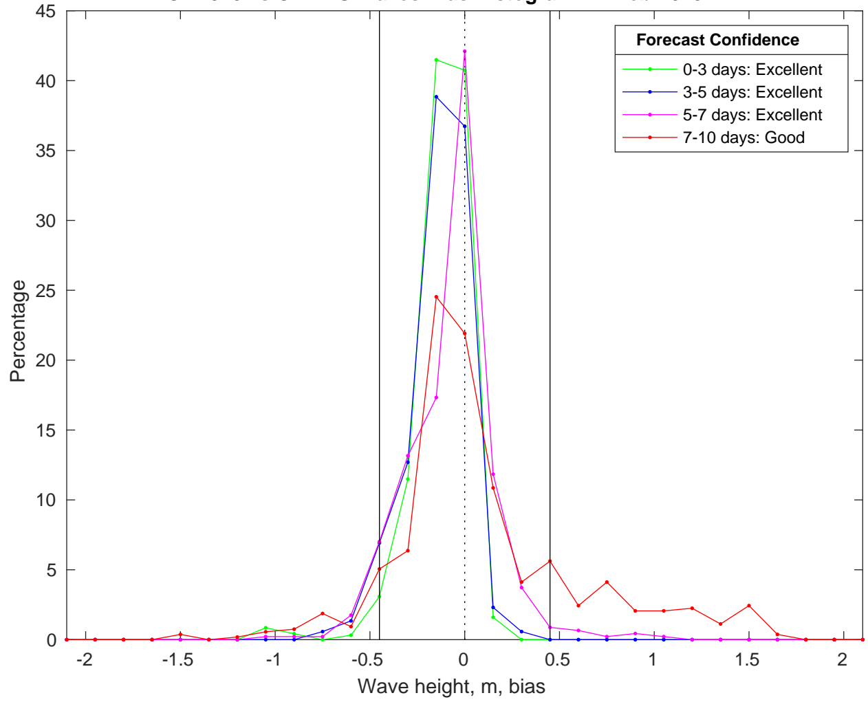
NDBC 42040 vs CMEMS Waves Bias Histogram: 11-Feb-2025
