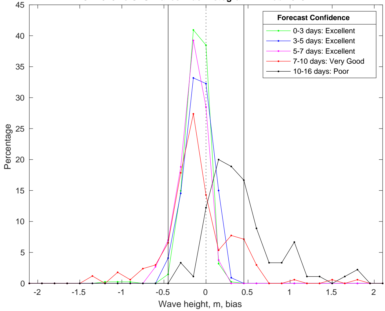
NDBC 42040 vs GFS Waves Bias Histogram: 11-Feb-2025
