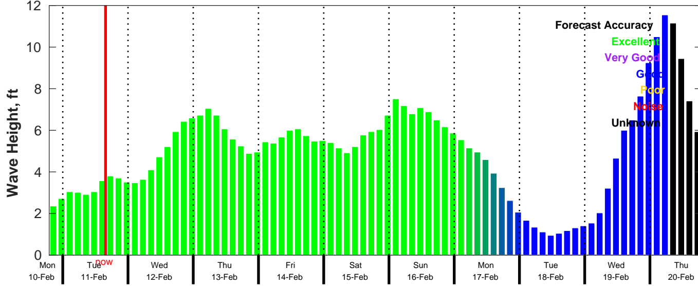
CMEMS Wave Forecast for NDBC 42040 from 10-Feb-2025 19:00:00 to 20-Feb-2025 19:00:00
