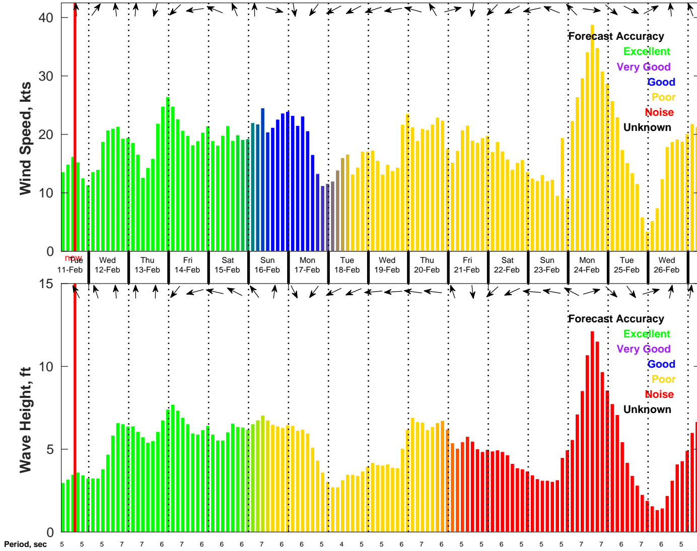
Wind & Wave Forecast for NDBC 42040 from 11-Feb-2025 07:00:00 to 27-Feb-2025 07:00:00
