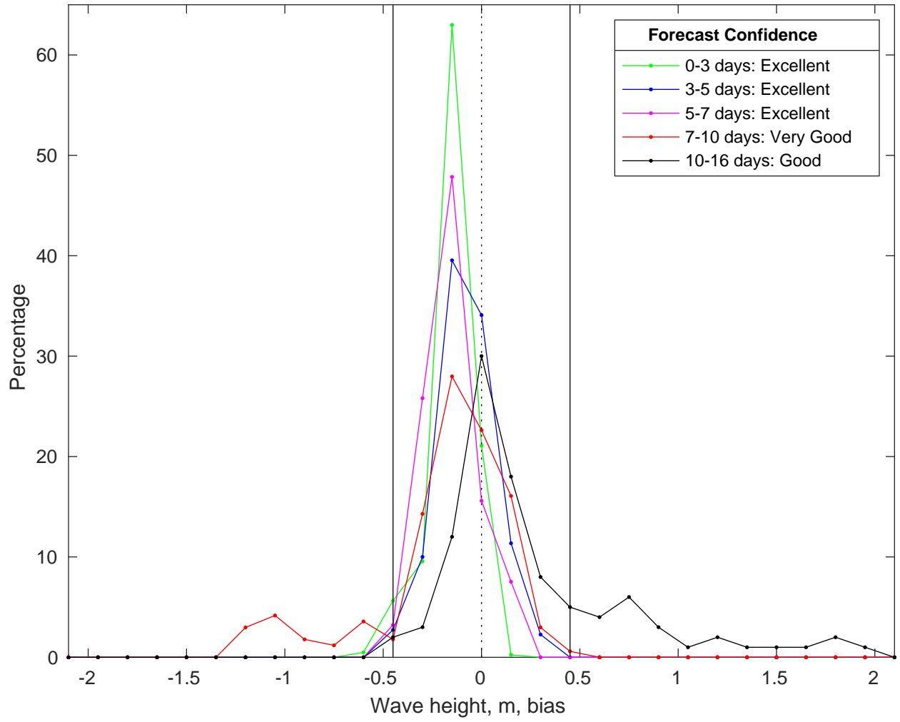
NDBC 42084 vs GFS Waves Bias Histogram: 11-Feb-2025
