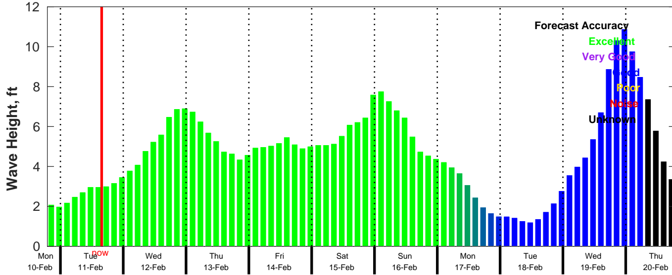
CMEMS Wave Forecast for NDBC 42084 from 10-Feb-2025 19:00:00 to 20-Feb-2025 19:00:00
