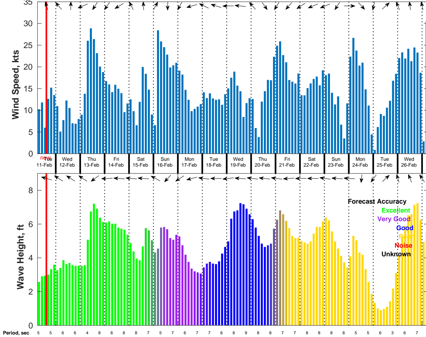
Wind & Wave Forecast for NDBC 42092 from 11-Feb-2025 06:00:00 to 27-Feb-2025 06:00:00
