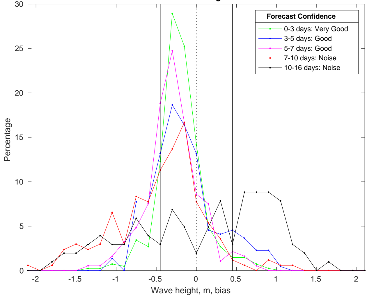
NDBC 46011 vs GFS Waves Bias Histogram: 11-Feb-2025
