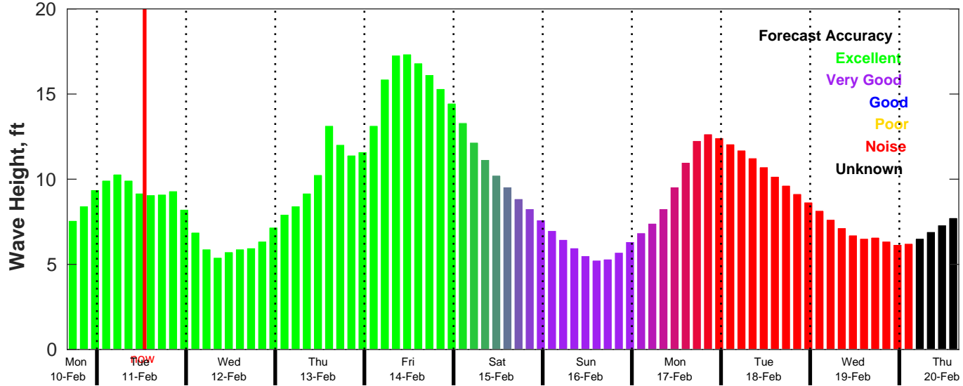
CMEMS Wave Forecast for NDBC 46011 from 10-Feb-2025 16:00:00 to 20-Feb-2025 16:00:00
