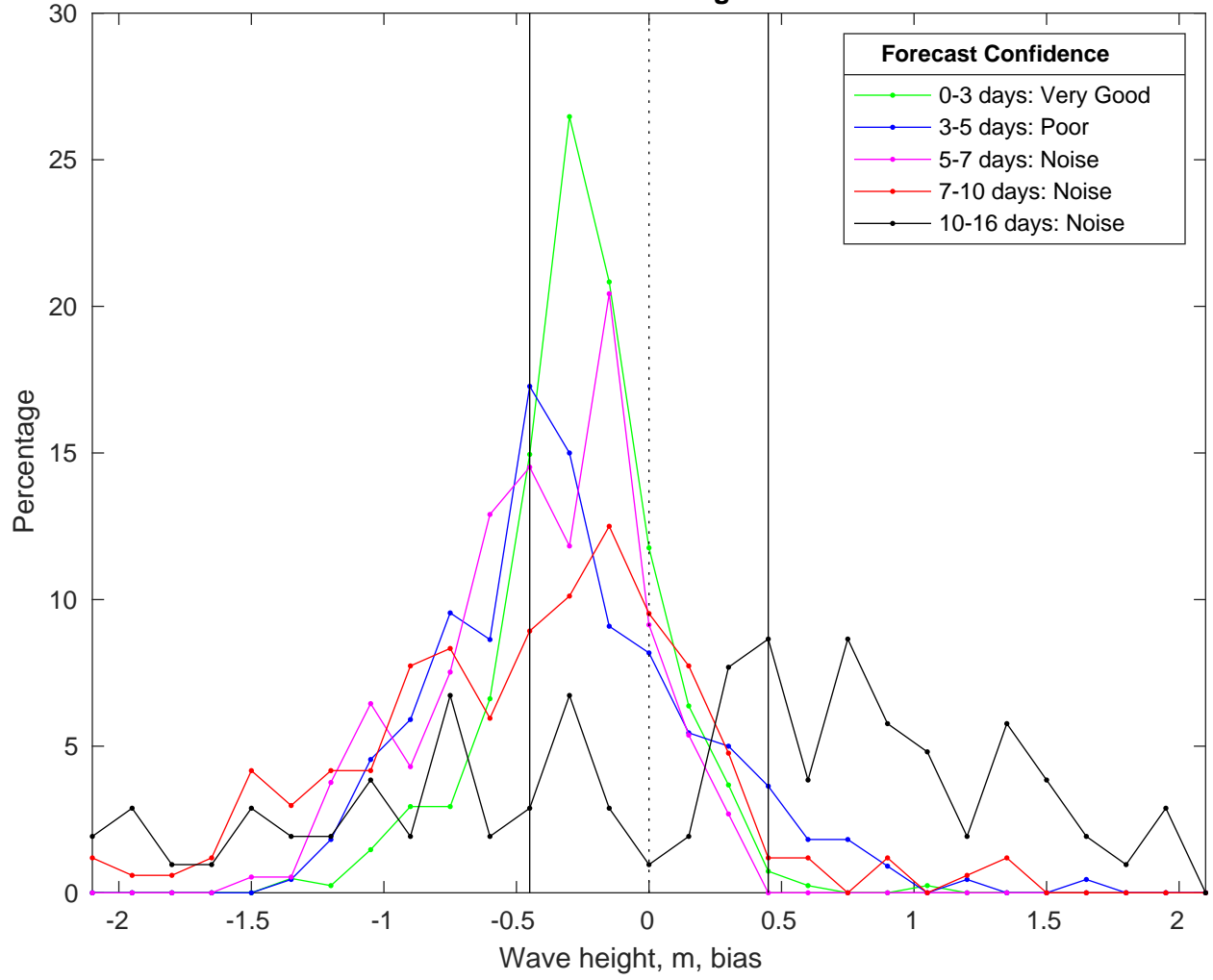
NDBC 46028 vs GFS Waves Bias Histogram: 11-Feb-2025
