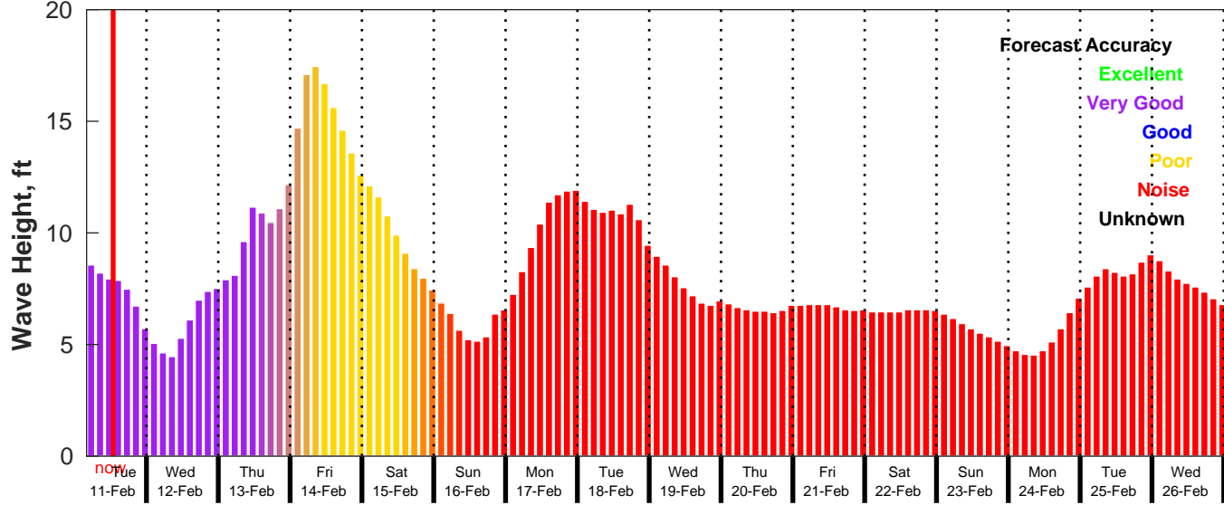
GFS Wave Forecast for NDBC 46028 from 11-Feb-2025 04:00:00 to 27-Feb-2025 04:00:00
