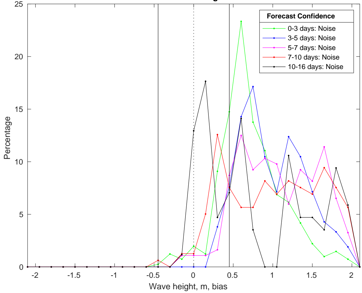
NDBC 46053 vs GFS Waves Bias Histogram: 11-Feb-2025
