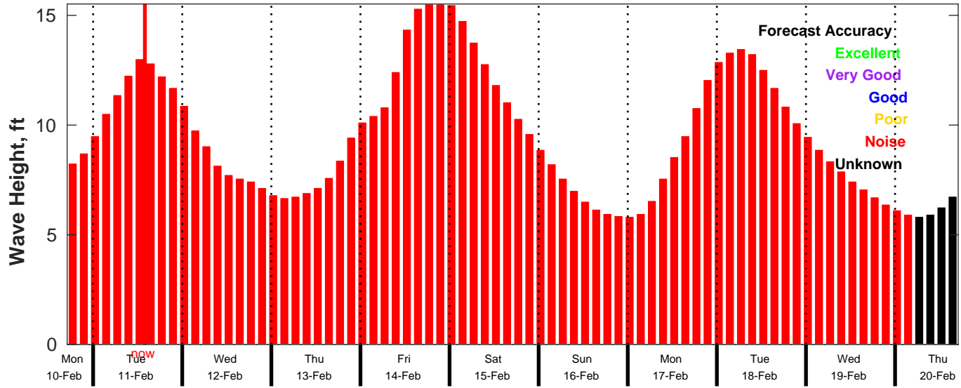
CMEMS Wave Forecast for NDBC 46053 from 10-Feb-2025 17:00:00 to 20-Feb-2025 17:00:00
