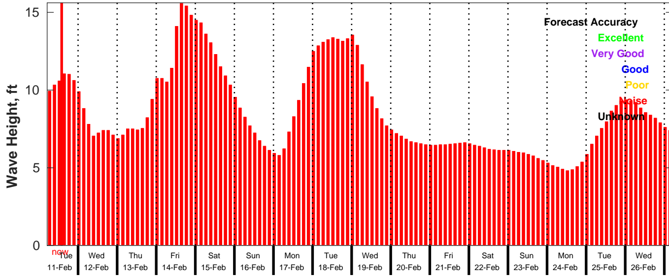
GFS Wave Forecast for NDBC 46053 from 11-Feb-2025 05:00:00 to 27-Feb-2025 05:00:00
