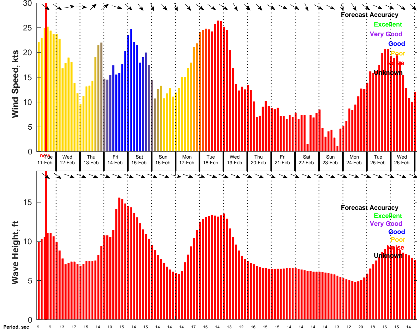
Wind & Wave Forecast for NDBC 46053 from 11-Feb-2025 05:00:00 to 27-Feb-2025 05:00:00
