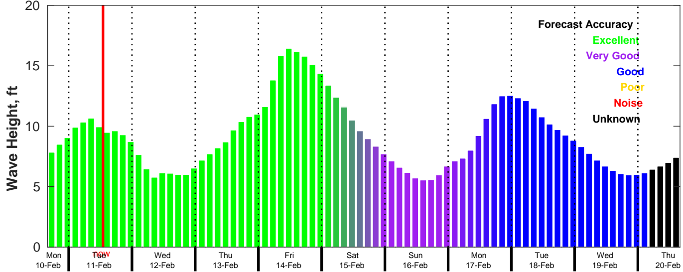
CMEMS Wave Forecast for NDBC 46054 from 10-Feb-2025 16:00:00 to 20-Feb-2025 16:00:00
