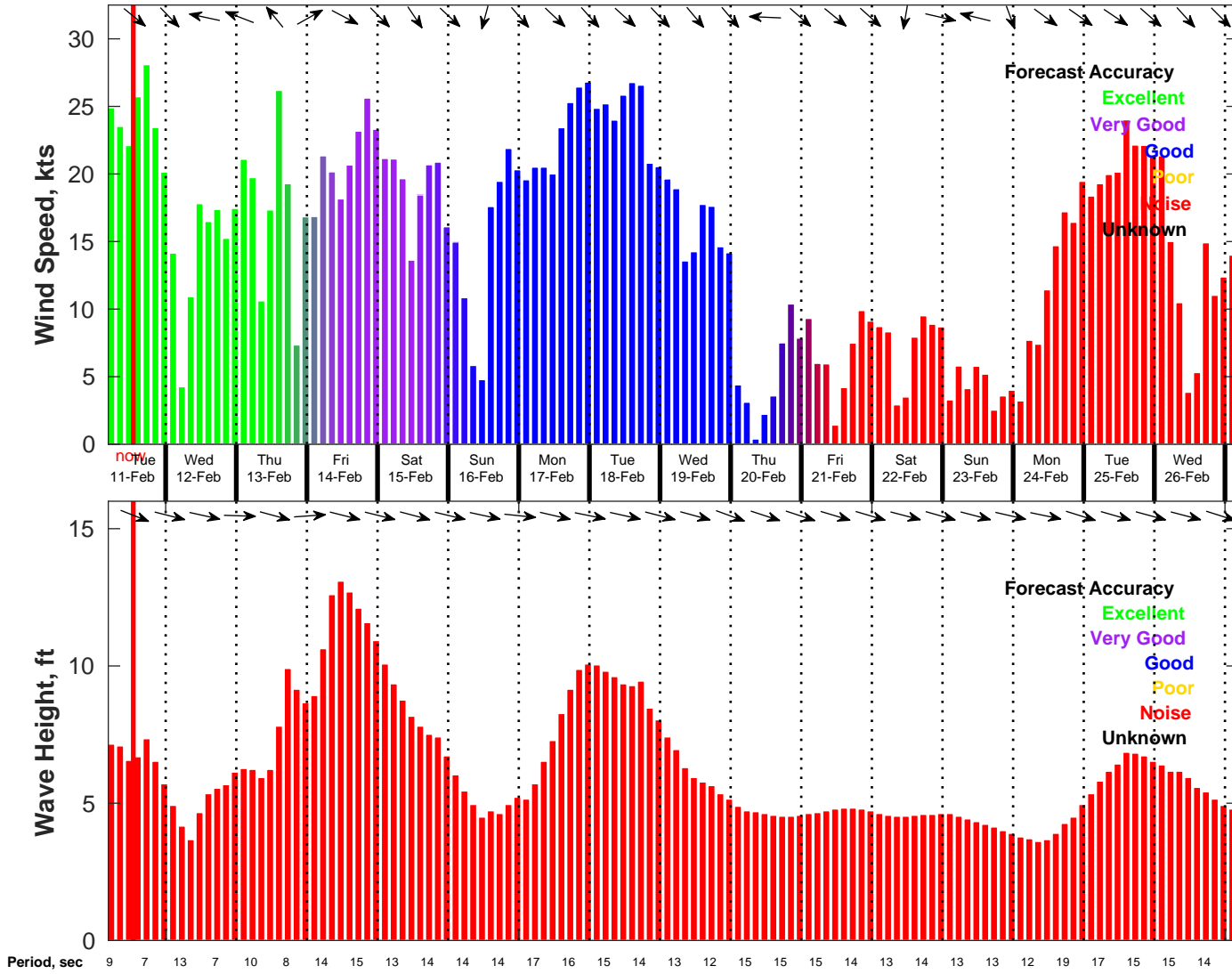
Wind & Wave Forecast for NDBC 46054 from 11-Feb-2025 04:00:00 to 27-Feb-2025 04:00:00
