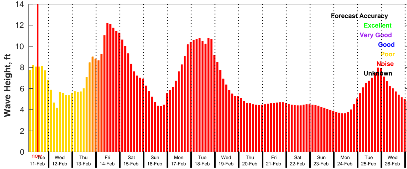
GFS Wave Forecast for NDBC 46069 from 11-Feb-2025 04:00:00 to 27-Feb-2025 04:00:00
