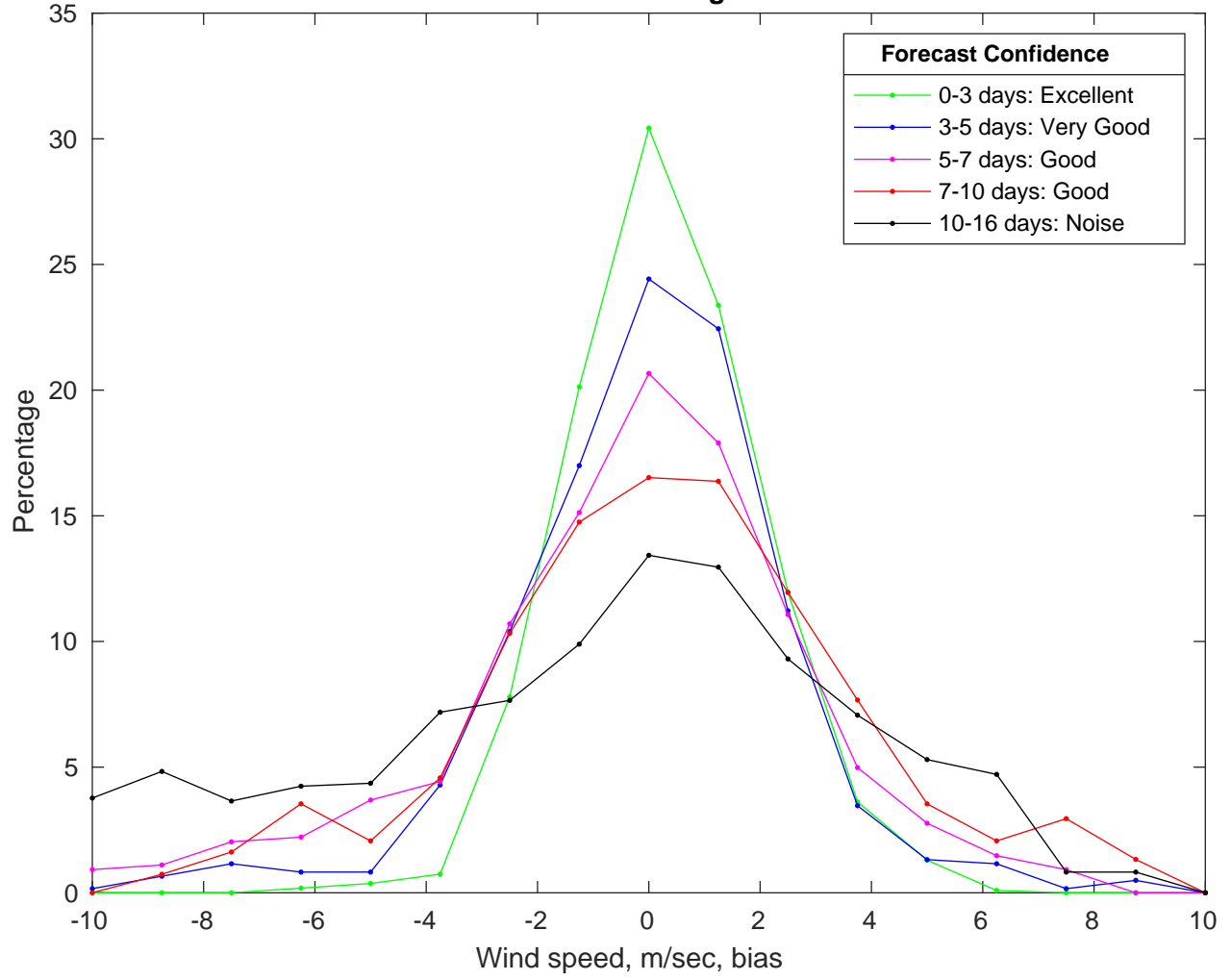
NDBC 46069 vs GFS Winds Bias Histogram: 26-Dec-2024
