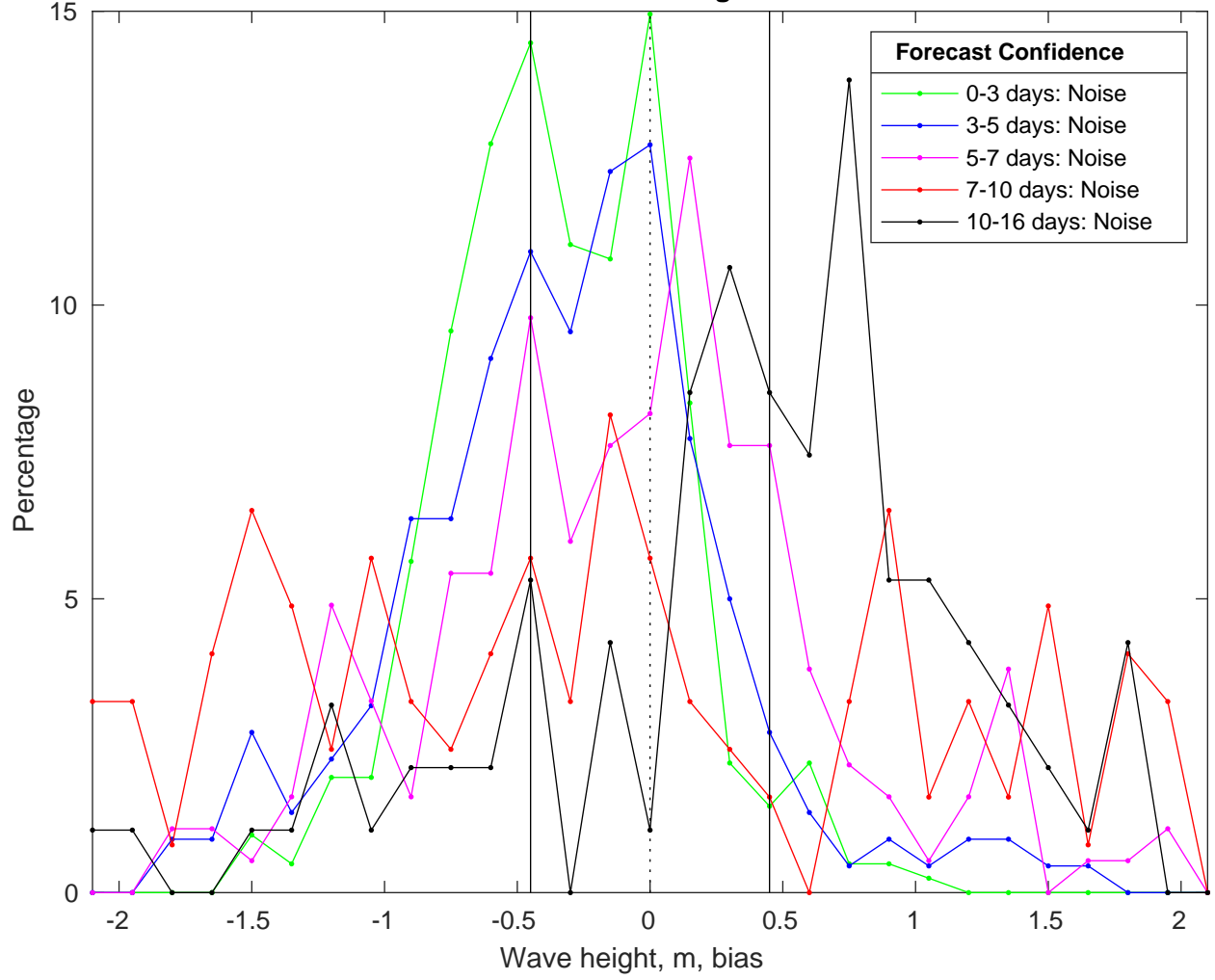
NDBC 46246 vs GFS Waves Bias Histogram: 11-Feb-2025
