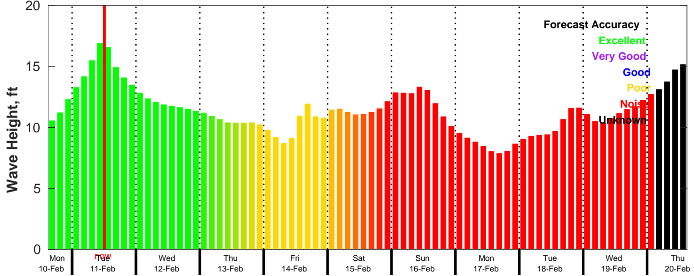
CMEMS Wave Forecast for NDBC 46246 from 10-Feb-2025 15:00:00 to 20-Feb-2025 15:00:00
