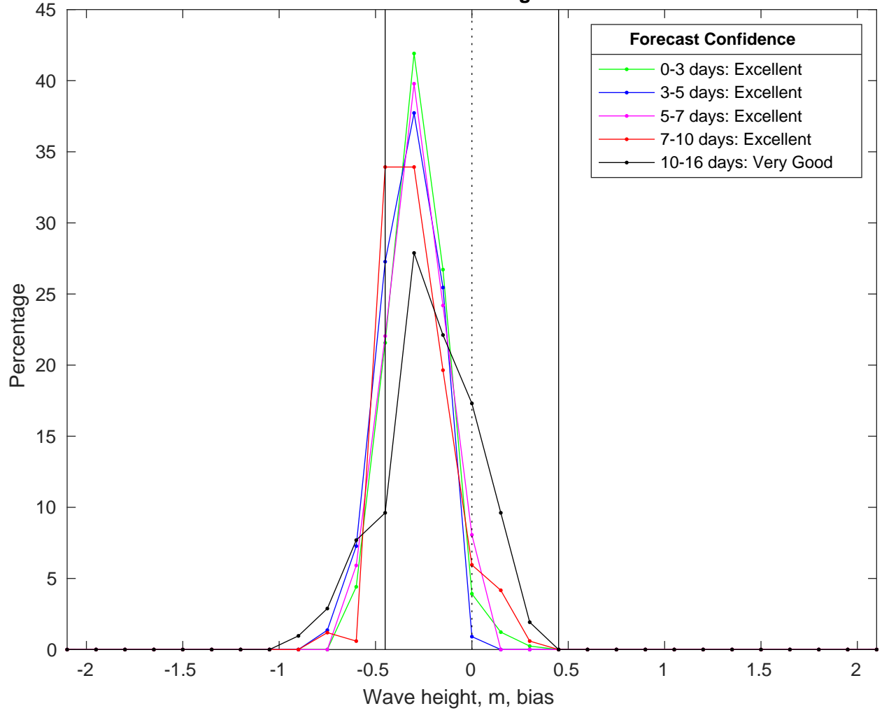
NDBC 51209 vs GFS Waves Bias Histogram: 11-Feb-2025
