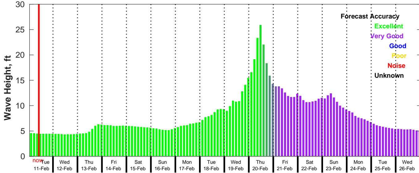
GFS Wave Forecast for NDBC 51209 from 11-Feb-2025 01:00:00 to 27-Feb-2025 01:00:00
