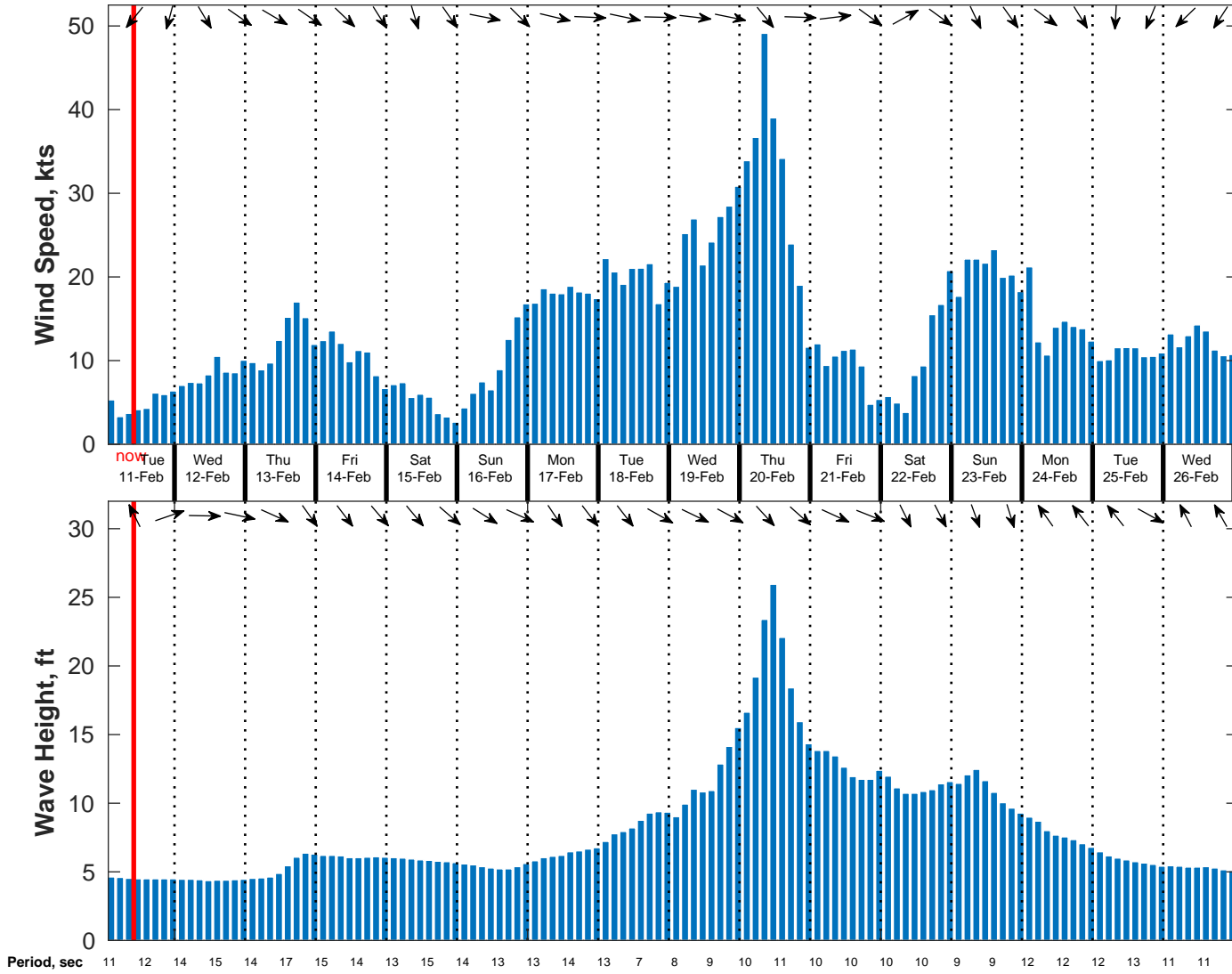
Wind & Wave Forecast for NDBC 51209 from 11-Feb-2025 01:00:00 to 27-Feb-2025 01:00:00
