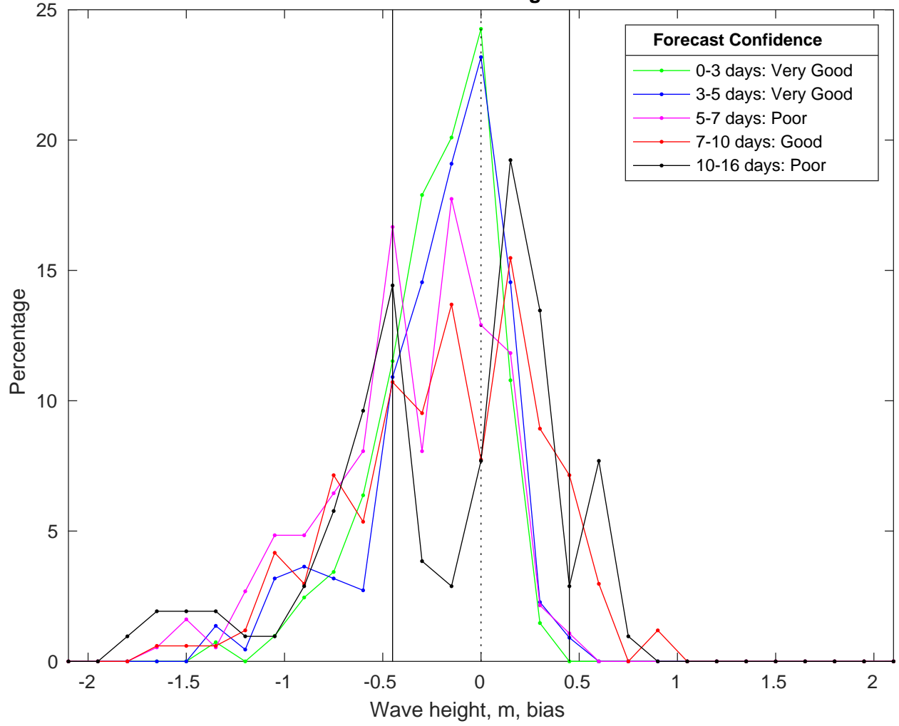
NDBC 52211 vs GFS Waves Bias Histogram: 11-Feb-2025
