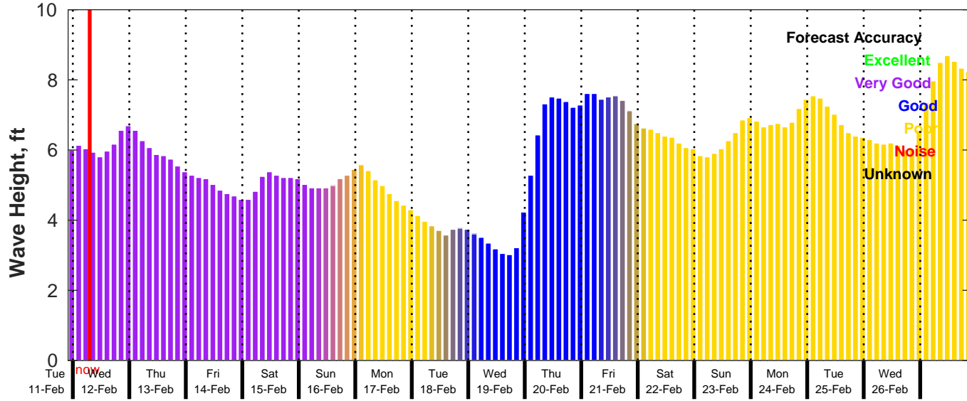
GFS Wave Forecast for NDBC 52211 from 11-Feb-2025 22:00:00 to 27-Feb-2025 22:00:00
