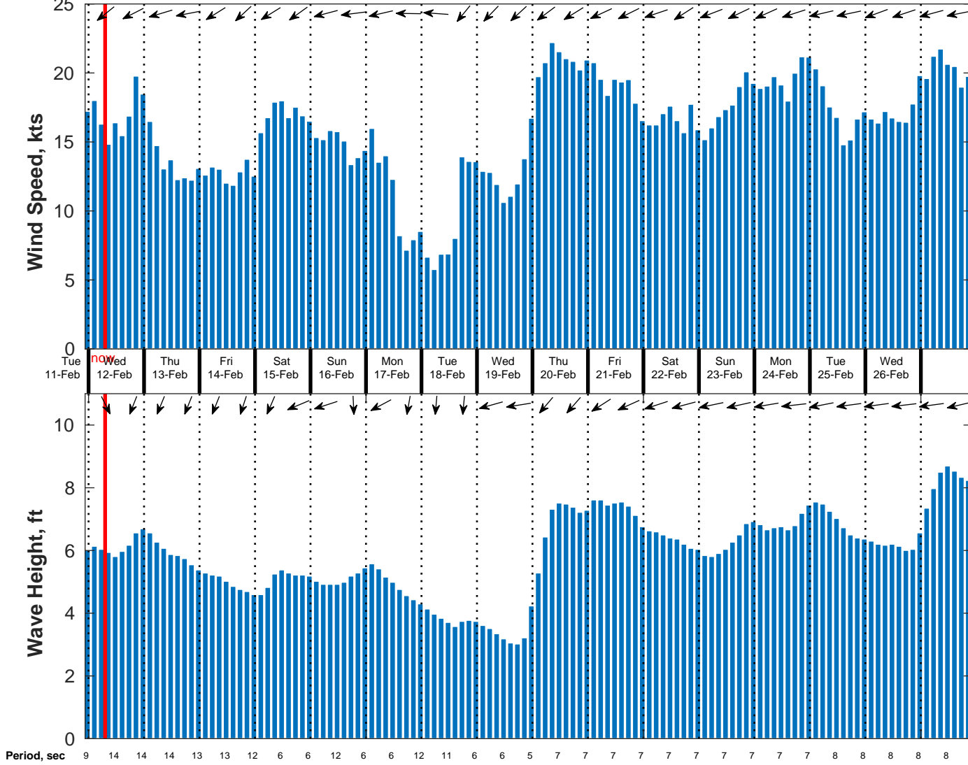
Wind & Wave Forecast for NDBC 52211 from 11-Feb-2025 22:00:00 to 27-Feb-2025 22:00:00
