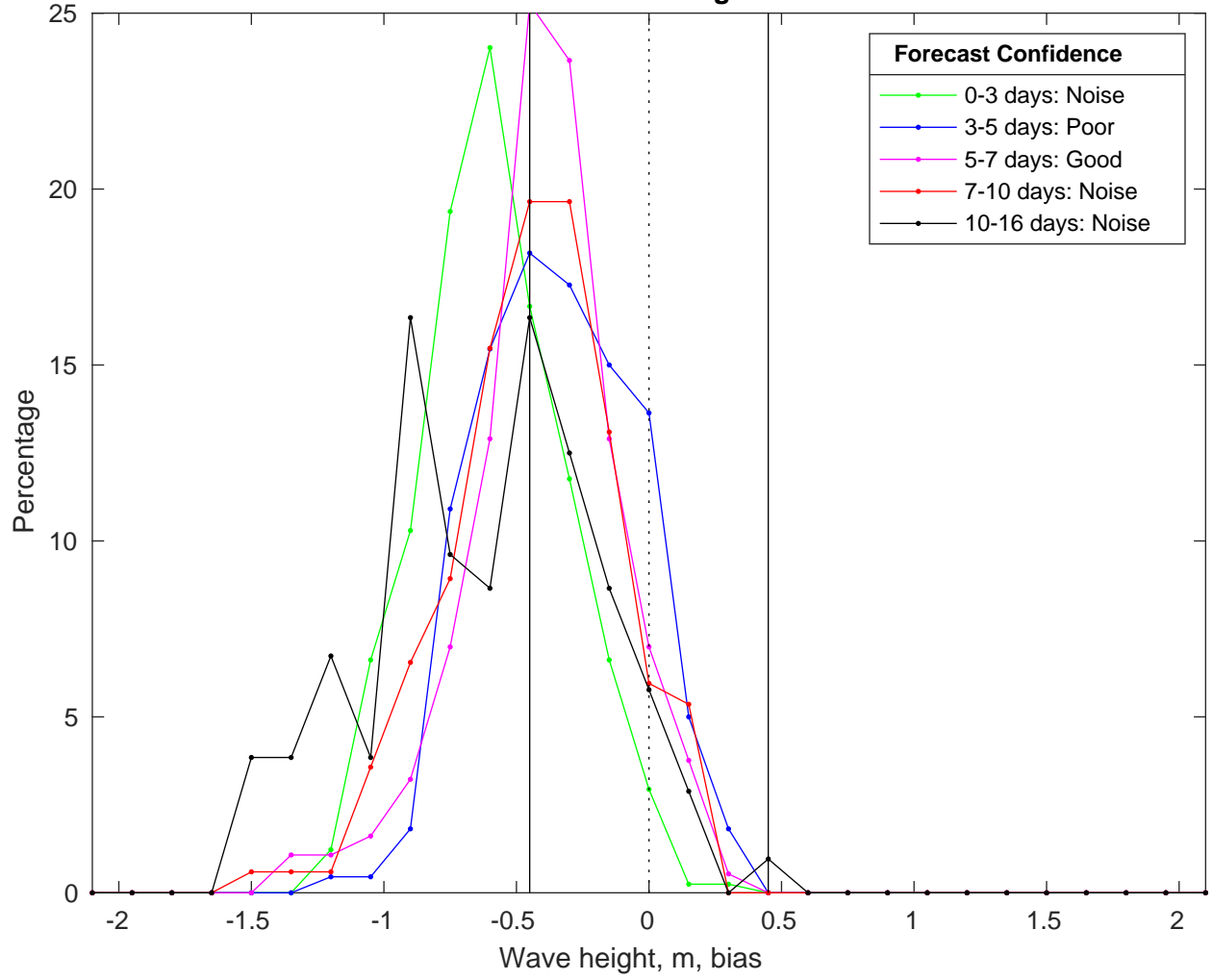
NDBC 52213 vs GFS Waves Bias Histogram: 11-Feb-2025
