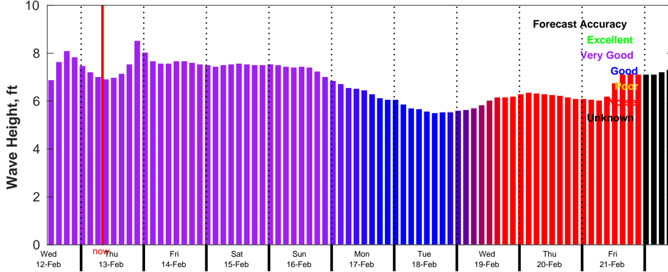
CMEMS Wave Forecast for NDBC 52213 from 11-Feb-2025 11:00:00 to 21-Feb-2025 11:00:00
