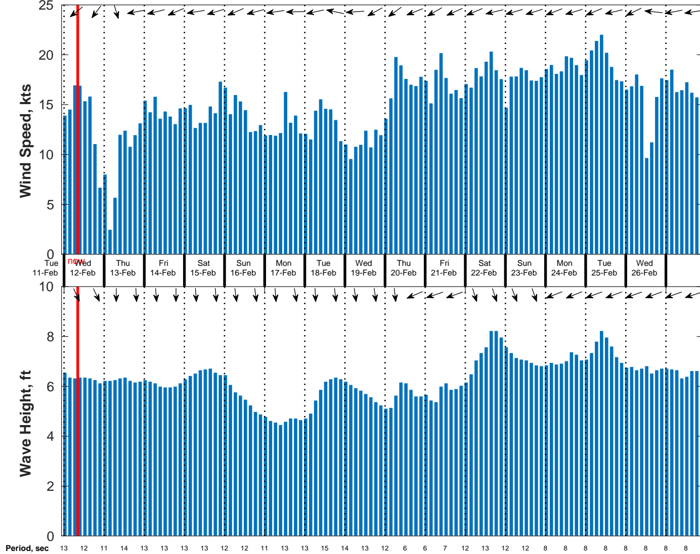
Wind & Wave Forecast for NDBC 52213 from 11-Feb-2025 23:00:00 to 27-Feb-2025 23:00:00
