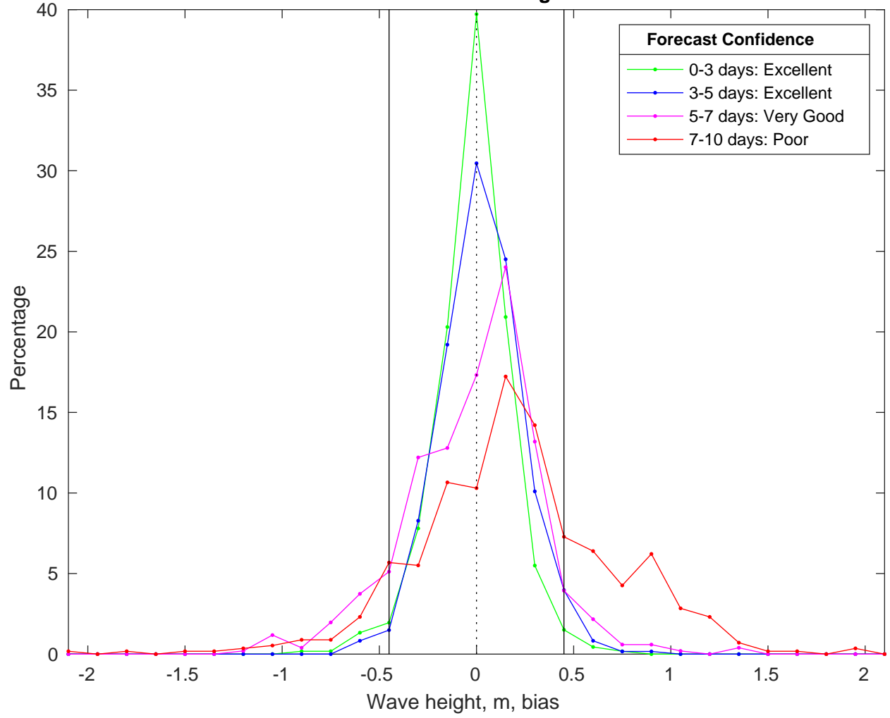
NDBC 41004 vs CMEMS Waves Bias Histogram: 12-Feb-2025
