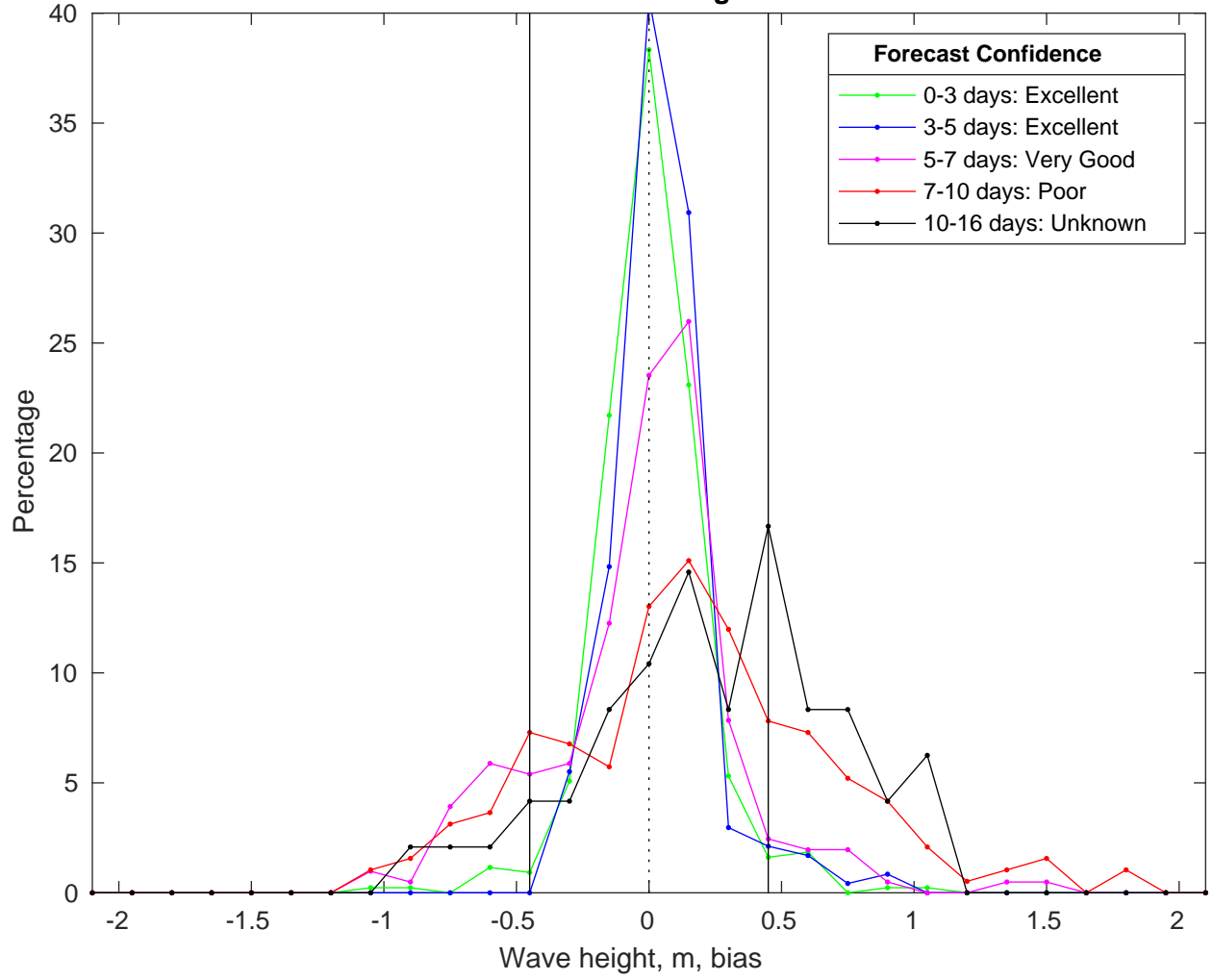
NDBC 41004 vs GFS Waves Bias Histogram: 12-Feb-2025
