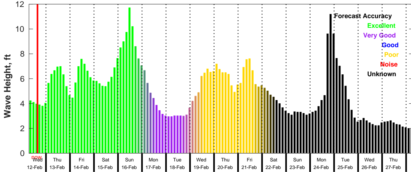
GFS Wave Forecast for NDBC 41004 from 12-Feb-2025 07:00:00 to 28-Feb-2025 07:00:00
