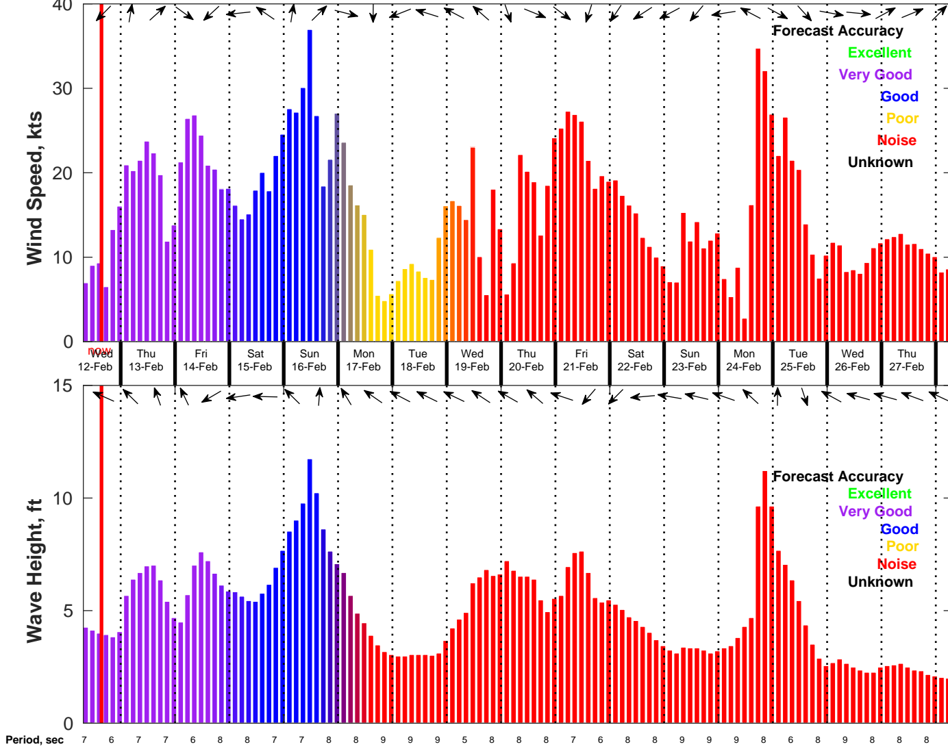
Wind & Wave Forecast for NDBC 41004 from 12-Feb-2025 07:00:00 to 28-Feb-2025 07:00:00
