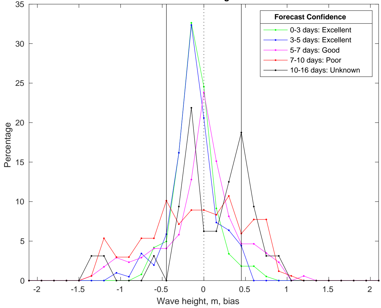
NDBC 41013 vs GFS Waves Bias Histogram: 12-Feb-2025
