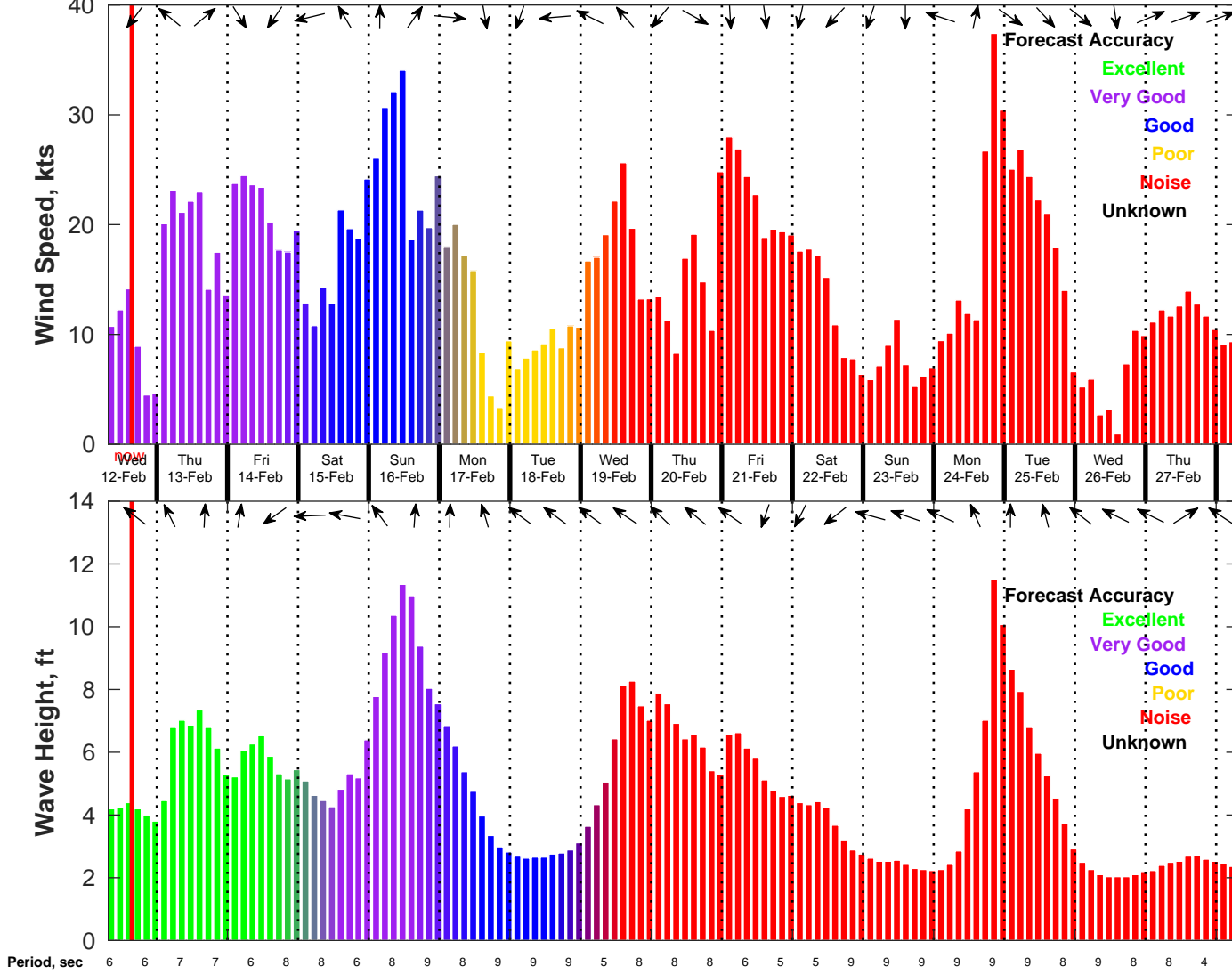
Wind & Wave Forecast for NDBC 41013 from 12-Feb-2025 07:00:00 to 28-Feb-2025 07:00:00
