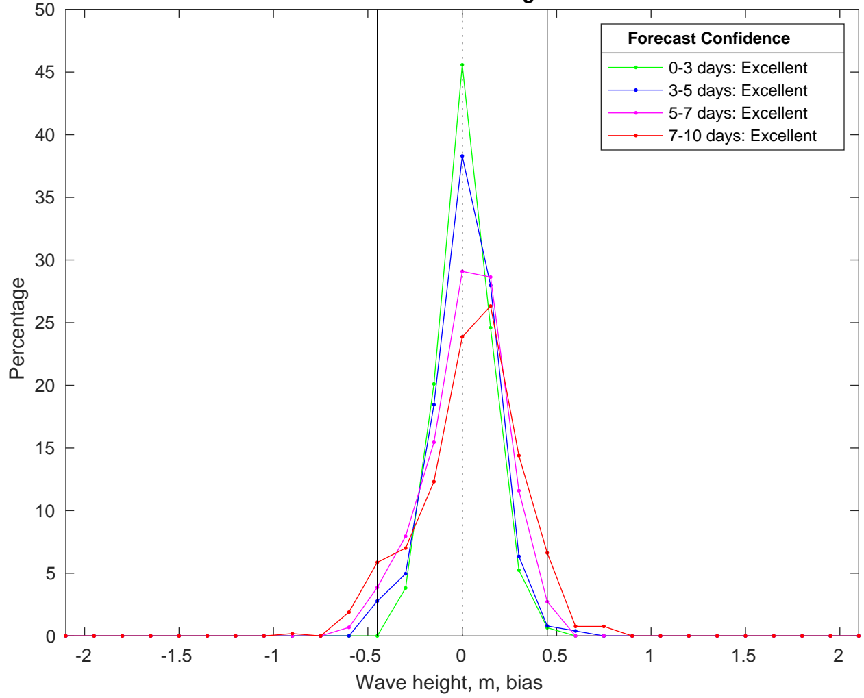
NDBC 41040 vs CMEMS Waves Bias Histogram: 12-Feb-2025
