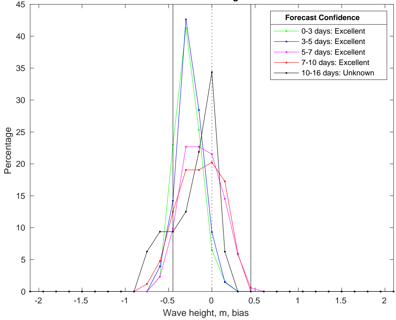
NDBC 41040 vs GFS Waves Bias Histogram: 12-Feb-2025
