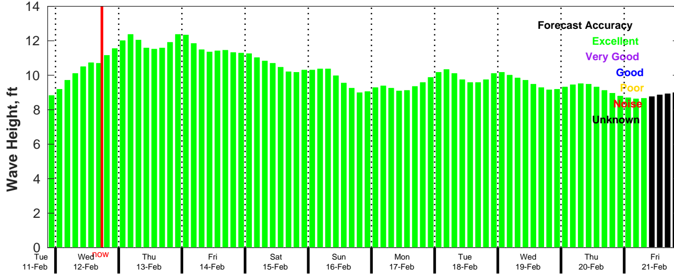
CMEMS Wave Forecast for NDBC 41040 from 11-Feb-2025 21:00:00 to 21-Feb-2025 21:00:00
