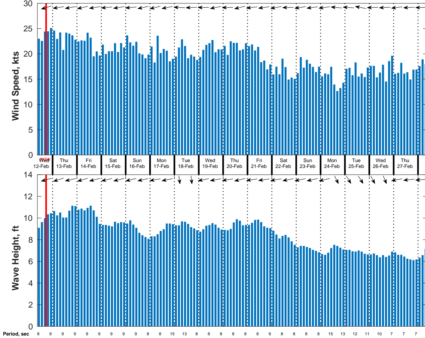
Wind & Wave Forecast for NDBC 41040 from 12-Feb-2025 09:00:00 to 28-Feb-2025 09:00:00
