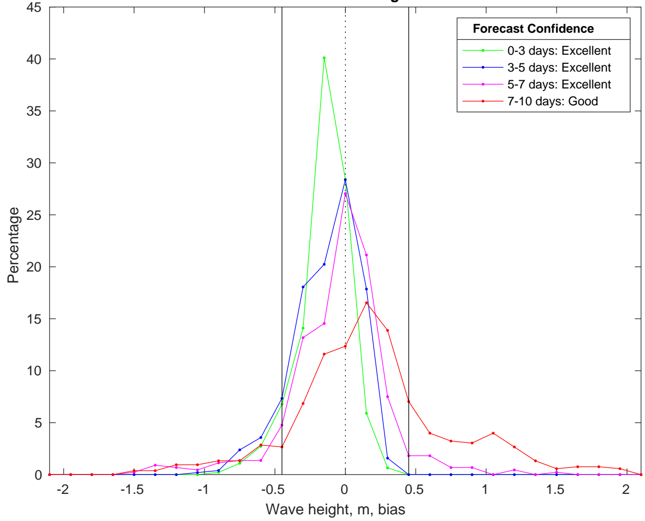
NDBC 42019 vs CMEMS Waves Bias Histogram: 12-Feb-2025
